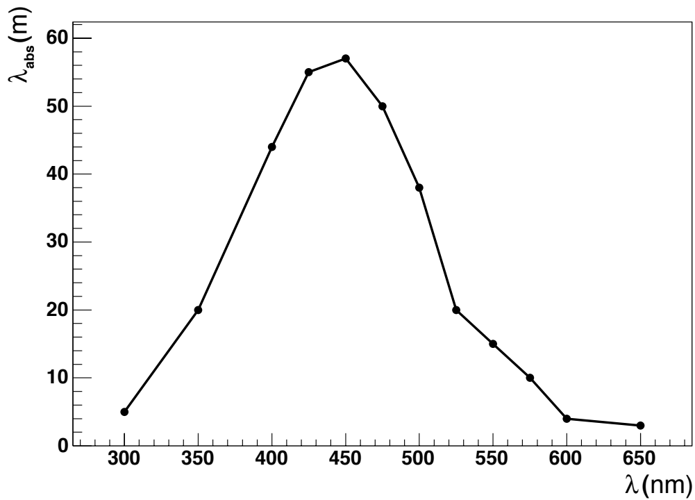
Figure 10: Light absorption length in sea water as a function of wavelength.
