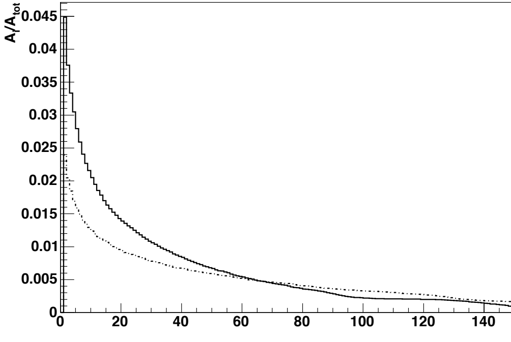
Figure 23: Average relative energy in the i -th non-zero cell when cells are ordered according to their energy content, for 800 MeV electrons (light) and muons (dark).
