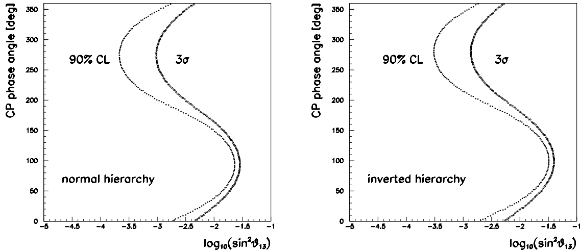
Figure 31: 90% CL and 3\sigma limits on \sin^2\theta_{13} as a function of the CP phase angle, for normal (left plot) and inverted (right plot) mass hierarchy.
