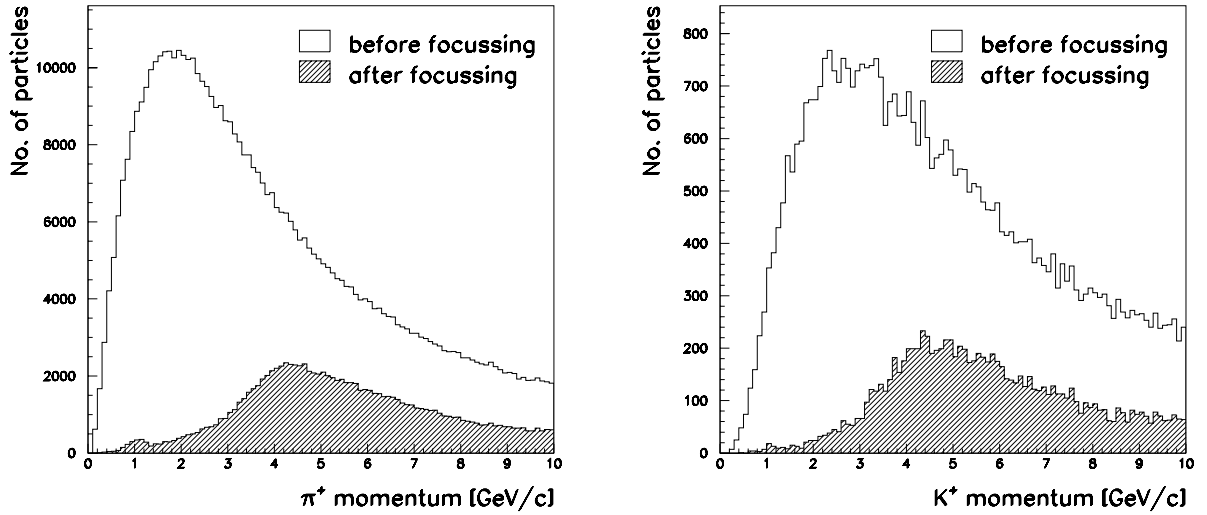
Figure 6: Momentum spectra of \pi^+ 's (left) and K^+ 's (right) before and after horn and reflector focusing.
