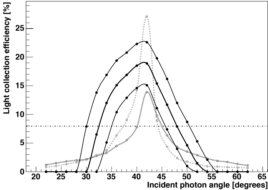
Figure 13: Angular response functions: the three continuous lines show the light collection efficiency of a parabolic mirror system with photodetectors with diameter 40, 50, and 60 cm, respectively; the horizontal line shows the geometrical light collection efficiency of 8% that was used in our simulations. For comparison, the angular incidences of photons from perpendicularly incident 800 MeV electrons (dotted, dark) and muons (dotted, light) are also shown.
