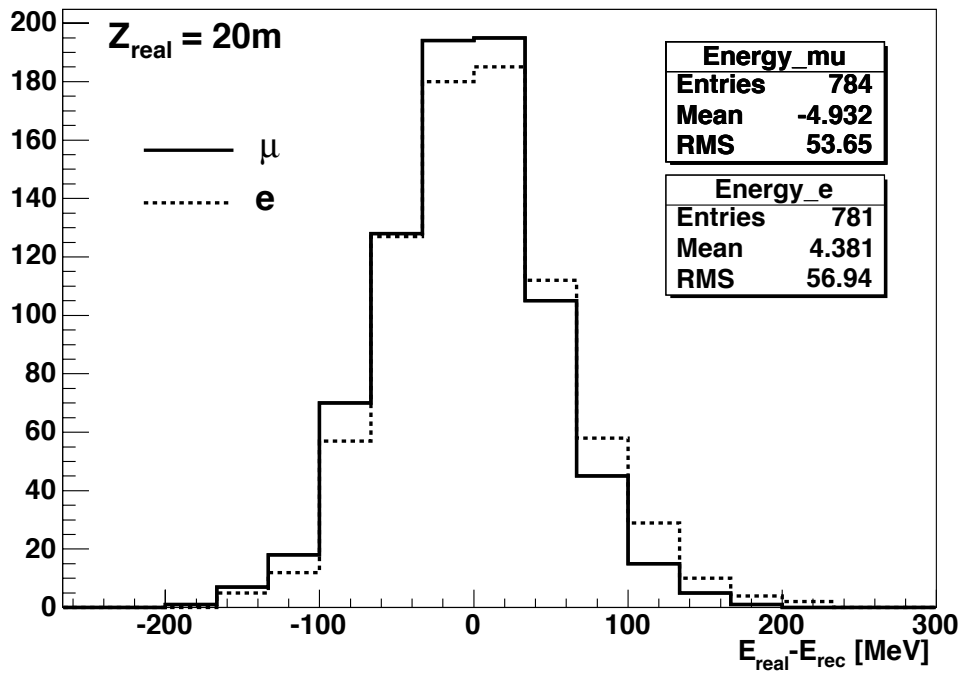
Figure 22: Energy resolution of 800 MeV electrons and muons.
