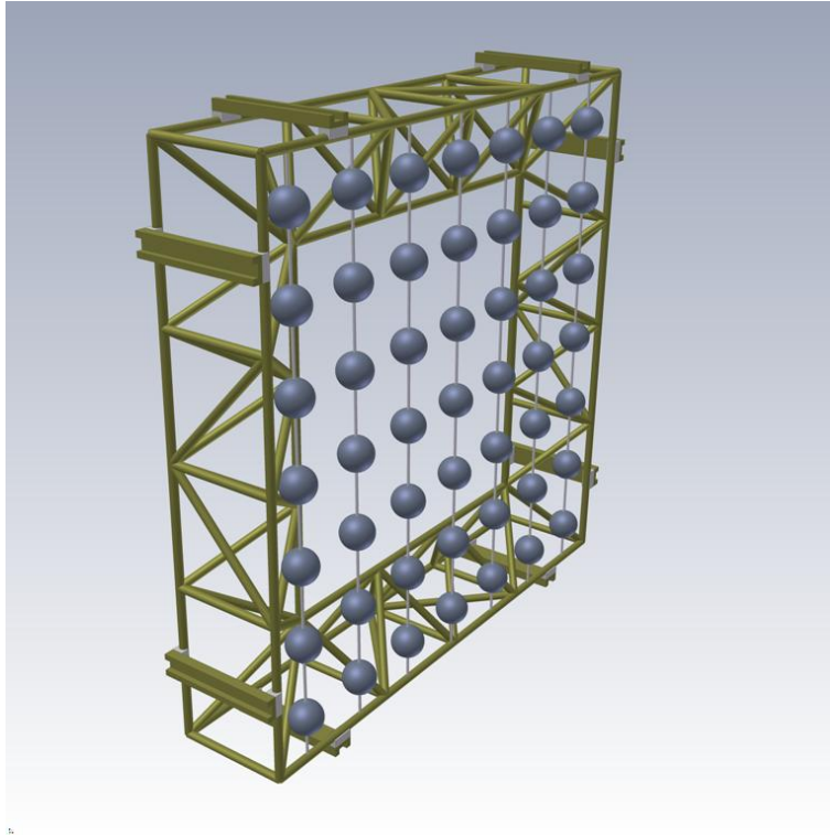
Figure 16: A 10 \times 10 \text{ m}^2 mechanical module with optical modules arranged in vertical strings; each side has two guides that locate the mechanical module with respect to the framework located between mechanical modules.
