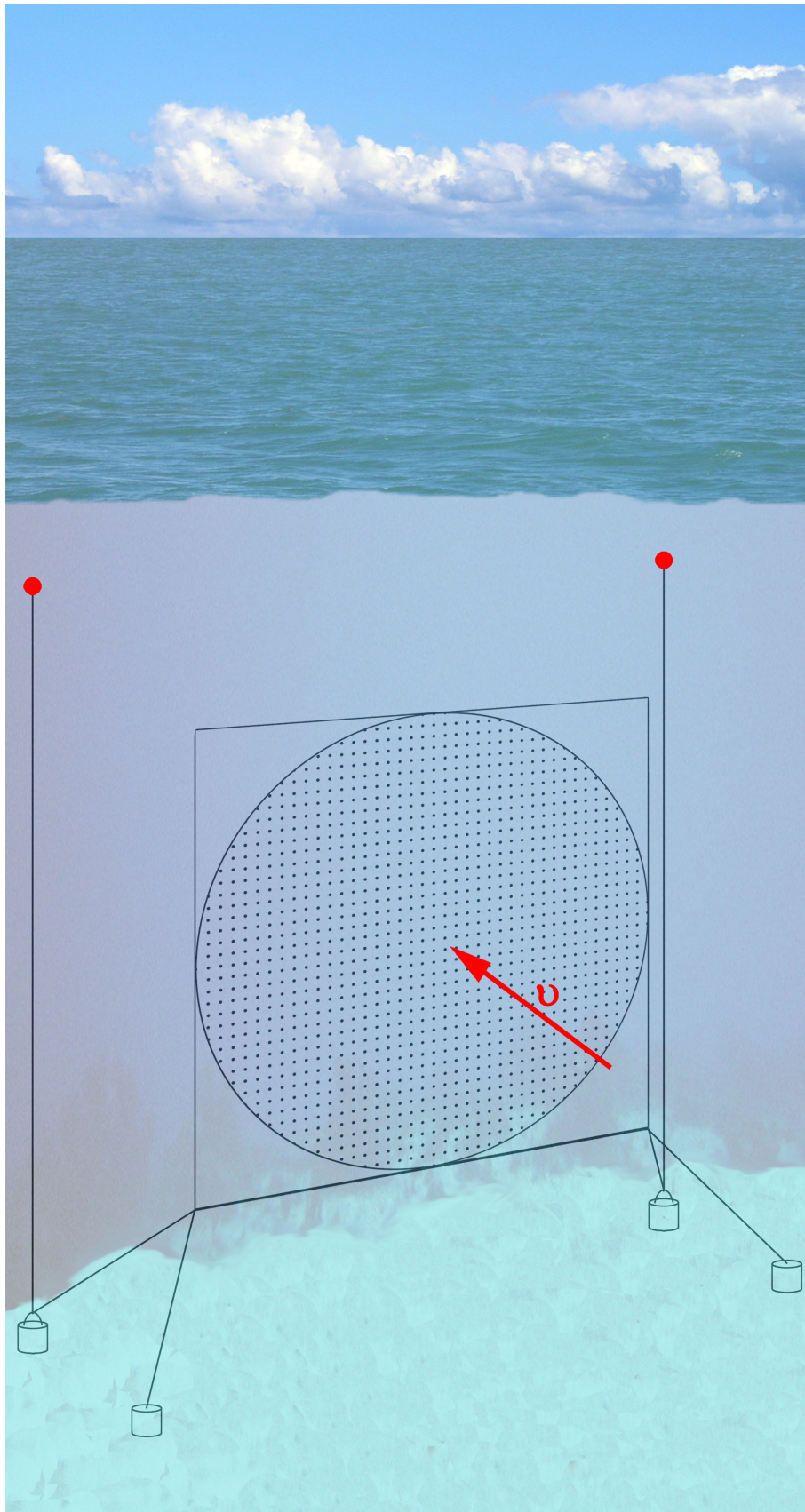
Figure 2: Schematic view of the underwater detector (not to scale), including the lower mooring system. The upper mooring system, which completes the stabilization of the structure, is not shown.
