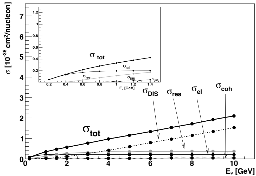
Figure 17: Charged-Current (top) and Neutral-Current (bottom) cross-sections per nucleon, as generated by NEUGEN, as a function of the neutrino energy. The subscripts ‘DIS’, ‘res’, ‘el’, and ‘coh’ refer to the deep-inelastic, resonant, elastic and coherent contributions, respectively. The inserts show the region of small neutrino energies, E_\nu < 1.5 GeV.
