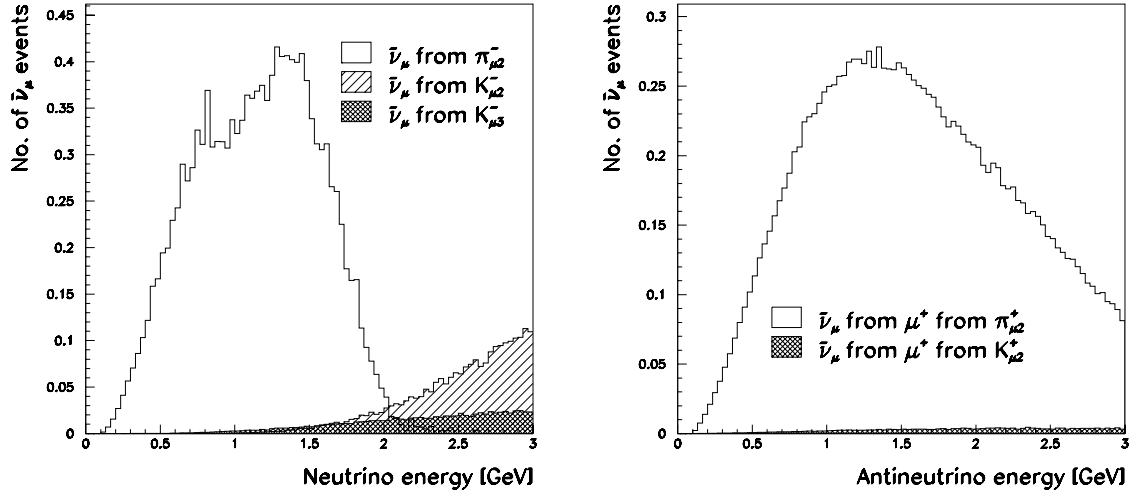
Figure 8: Momentum spectra (before oscillations) of \bar{\nu}_\mu events from \pi^- and K^- decays (left), and of \bar{\nu}_\mu events from \mu^+ 's originating from \pi^+ and K^+ decays (right). \bar{\nu}_\mu events from \mu^+ 's originating from K_{\mu 3}^+ decays are not shown because they would be hardly visible on this scale.
