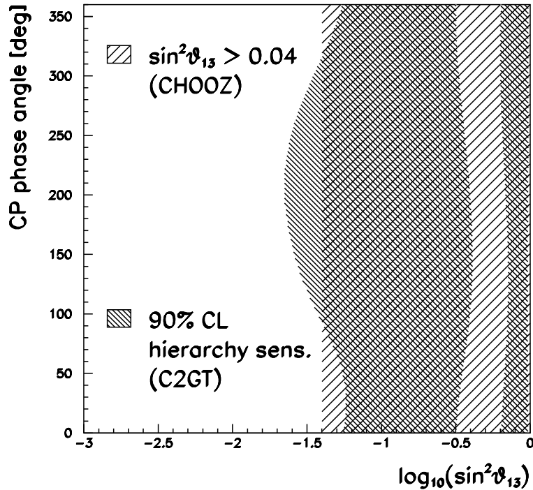
Figure 32: 90% confidence level region on the mass hierarchy.
