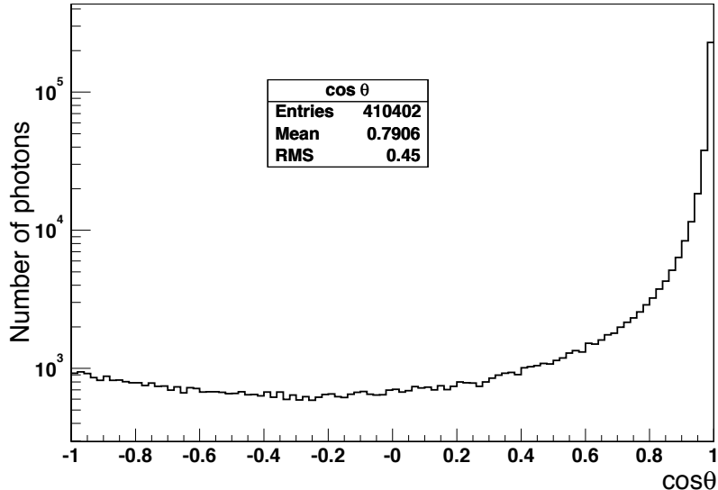
Figure 12: The cosine of photon scattering angle in sea water, showing the superposition of forward–backward symmetric Rayleigh scattering and forward Mie scattering.
