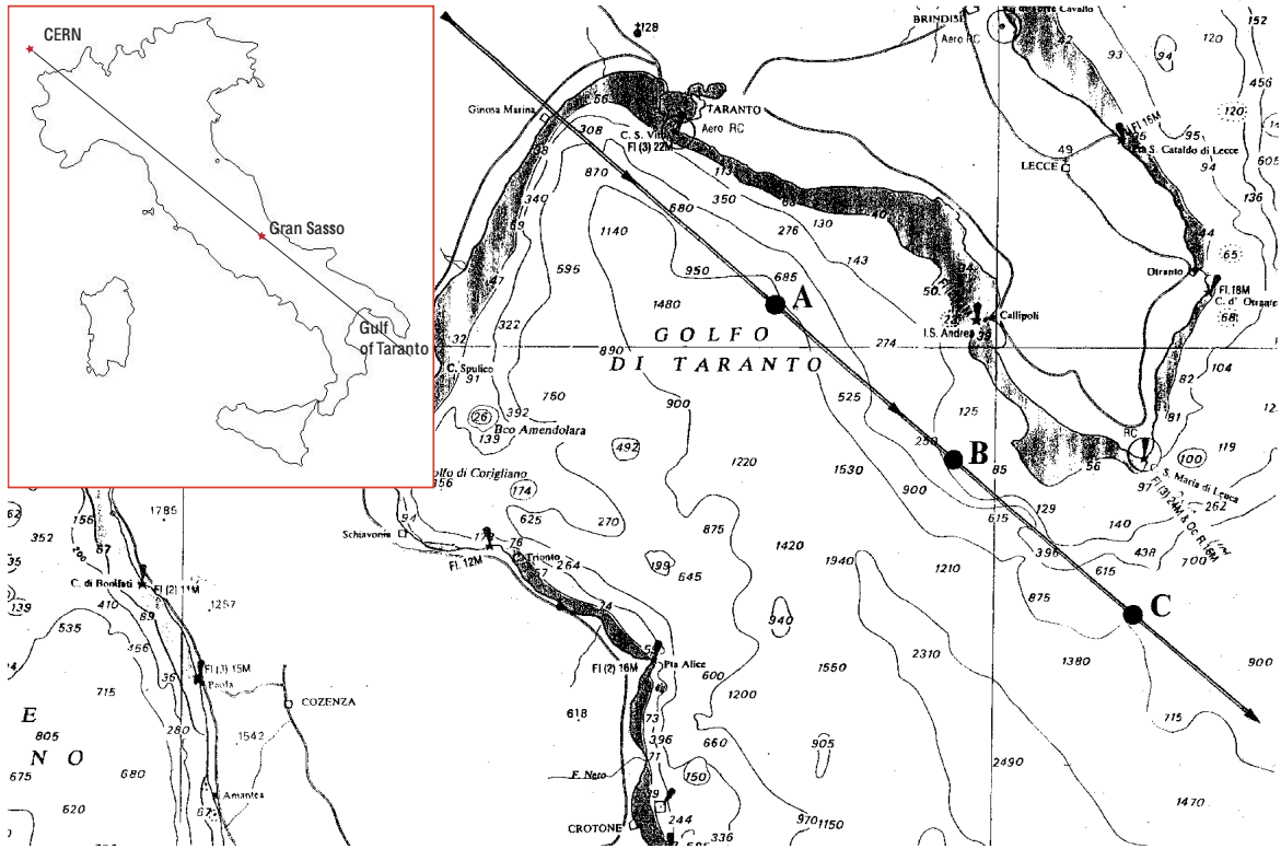
Figure 1: Chart of the Gulf of Taranto. The axis of the CNGS is shown as a solid line. For orientation, the points A, B, and C show locations separated by 50 km, with B at a distance of 1200 km from CERN. In practice, the C2GT detector would be located slightly south-west of the line, i.e., at positions that are not exactly vertical below the beam axis.
