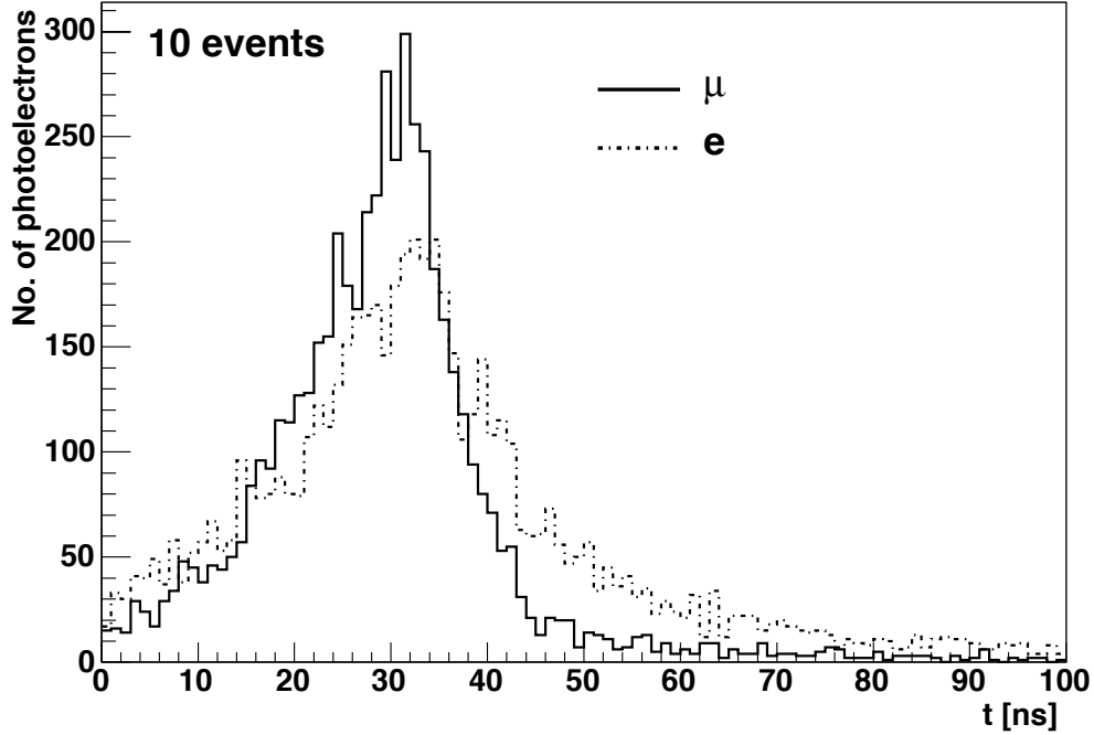
Figure 20: Time distribution of the arrival of photons from 800 MeV electrons and muons from a vertex located 20 m upstream of the detector plane.
