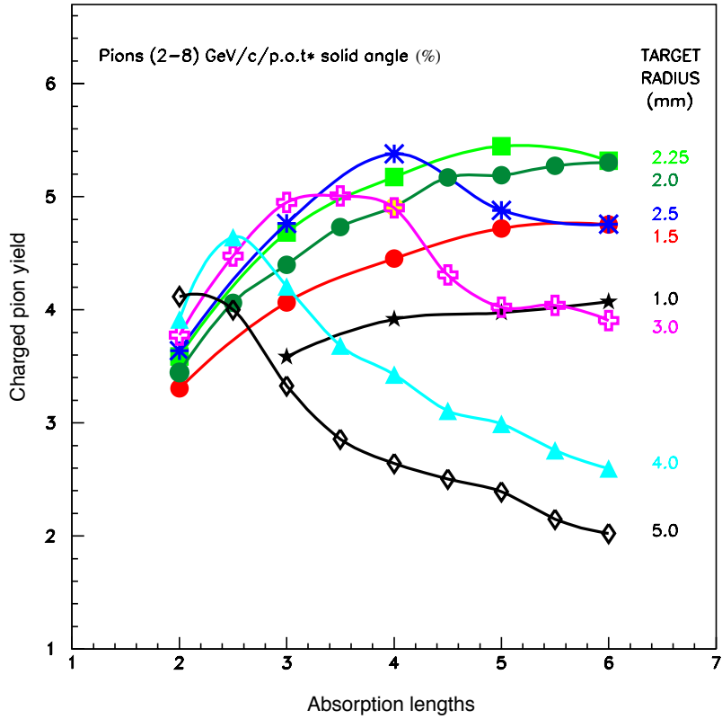
Figure 4: Yield of \pi^\pm 's from rotationally symmetric graphite targets with different absorption lengths and radii.
