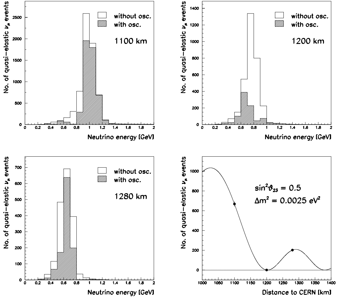
Figure 29: Charged-Current quasi-elastic \nu_\mu spectra at the three baselines of 1100, 1200 and 1280 km; the right lower plot shows a fit of the quasi-elastic event rates in terms of the oscillation parameters \sin^2 \theta_{23} and \Delta m_{23}^2 .
