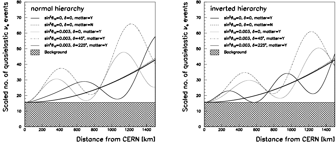
Figure 30: Charged-Current quasi-elastic \nu_e event numbers as a function of the distance from CERN, scaled to the nominal distance of 1200 km; event numbers for various sets of oscillation parameters are shown, for normal mass hierarchy (left plot) and for inverted hierarchy (right plot).
