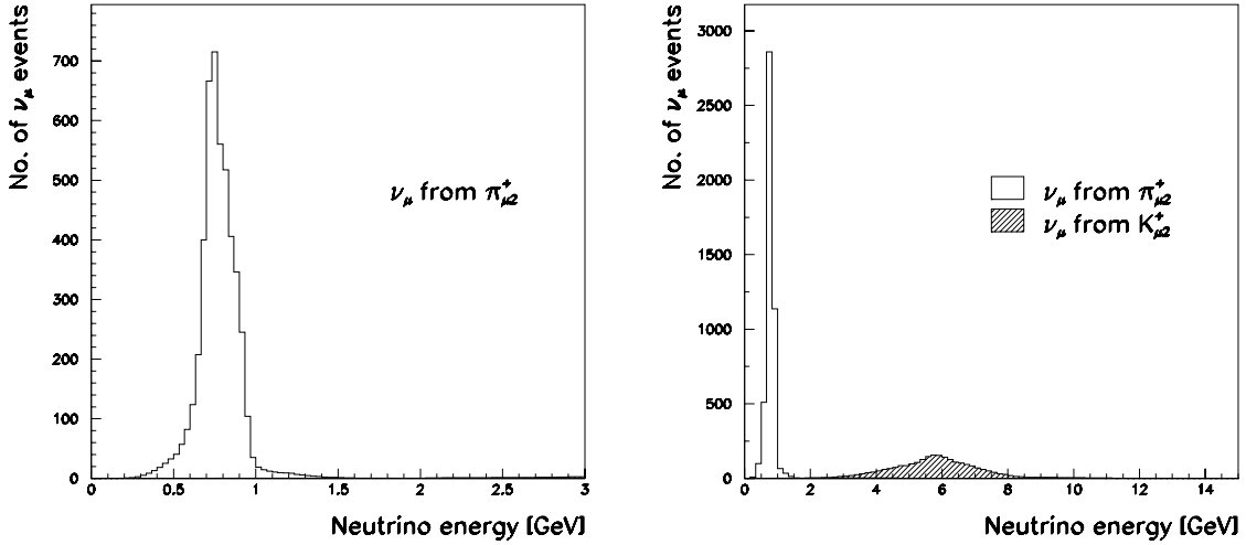
Figure 7: Momentum spectra (before oscillations) of \nu_\mu events from \pi^+ and K^+ decays. The left plot shows the momentum spectrum of \nu_\mu events from \pi^+ decays in more detail; the \nu_\mu events from K^+ decays are hardly visible on this scale.
