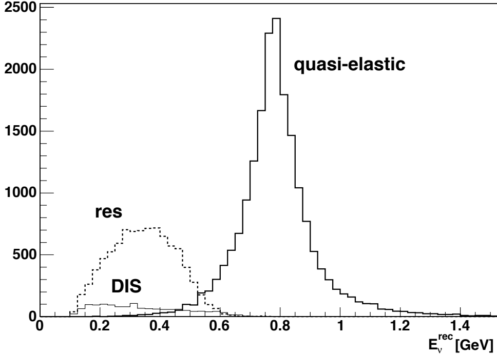
Figure 26: Neutrino energy reconstructed from events with a single muon under the hypothesis of quasi-elastic neutrino–nucleon scattering.
