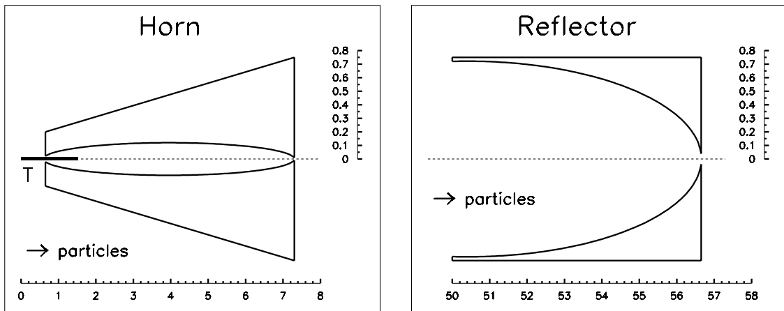
Figure 5: Longitudinal profiles of the horn (left) and the reflector (right). The location of the target T with respect to the horn is also shown. All scales are in metres.
