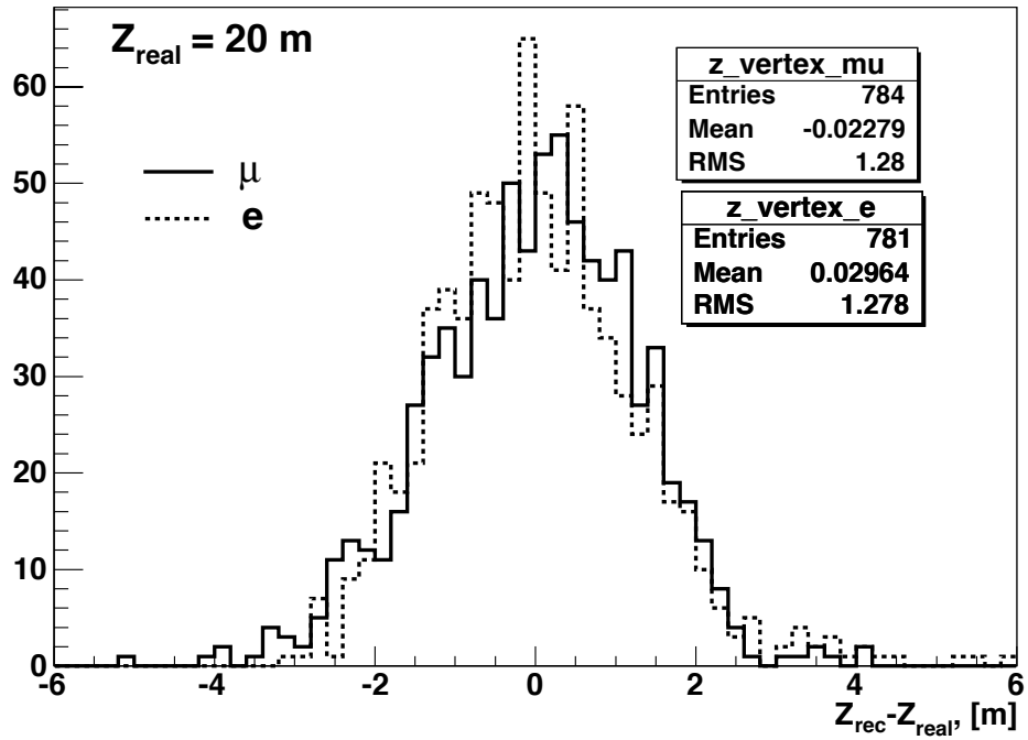
Figure 21: Difference between reconstructed and generated longitudinal vertex coordinate for 800 MeV electrons and muons.
