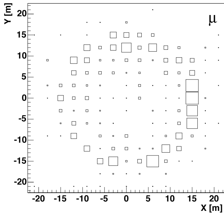
Figure 19: Cherenkov rings in terms of photoelectrons of a typical electron (top) and muon (bottom) event with 800 MeV total energy, with the vertex located 20 m upstream of the detector plane.
