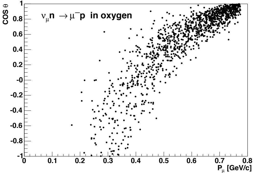
Figure 25: Cosine of the polar angle of muons from the quasi-elastic reaction in the ^{16}\text{O} nucleus, versus muon momentum.
